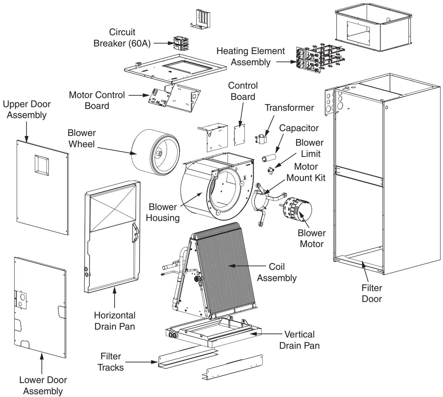
Air Handler Components
