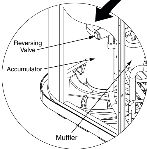
Refrigerant Valve (SM)
