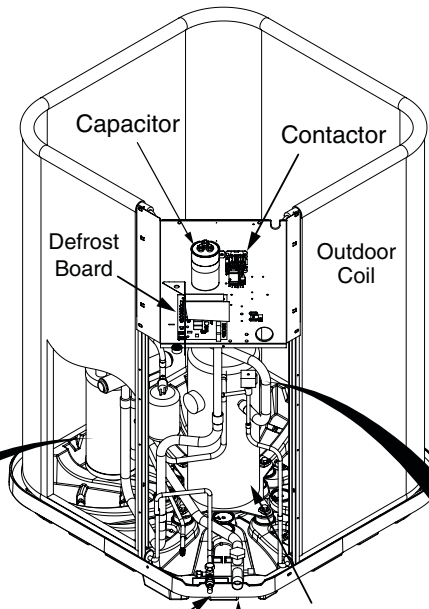
Compressor
