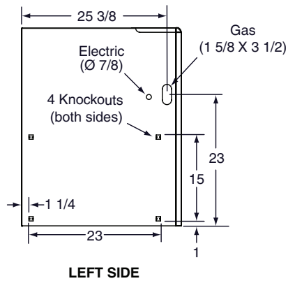
KG7TA Upflow/Horizontal Series
