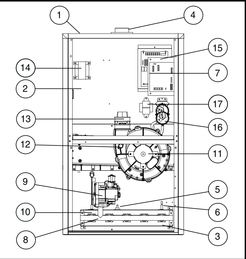
Downflow Gas Furnace
