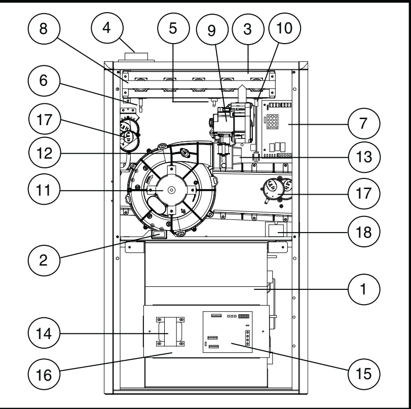
Upflow/Horizontal Gas Furnace
