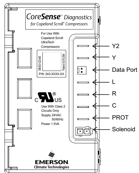
Figure 2 Terminal Locations
