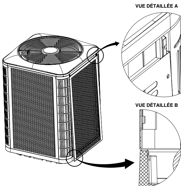
Figure 5. Installation du panneau
